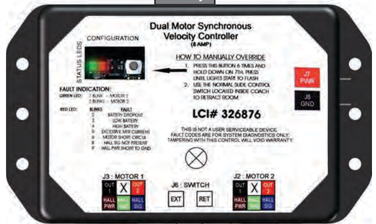
8 Amp
